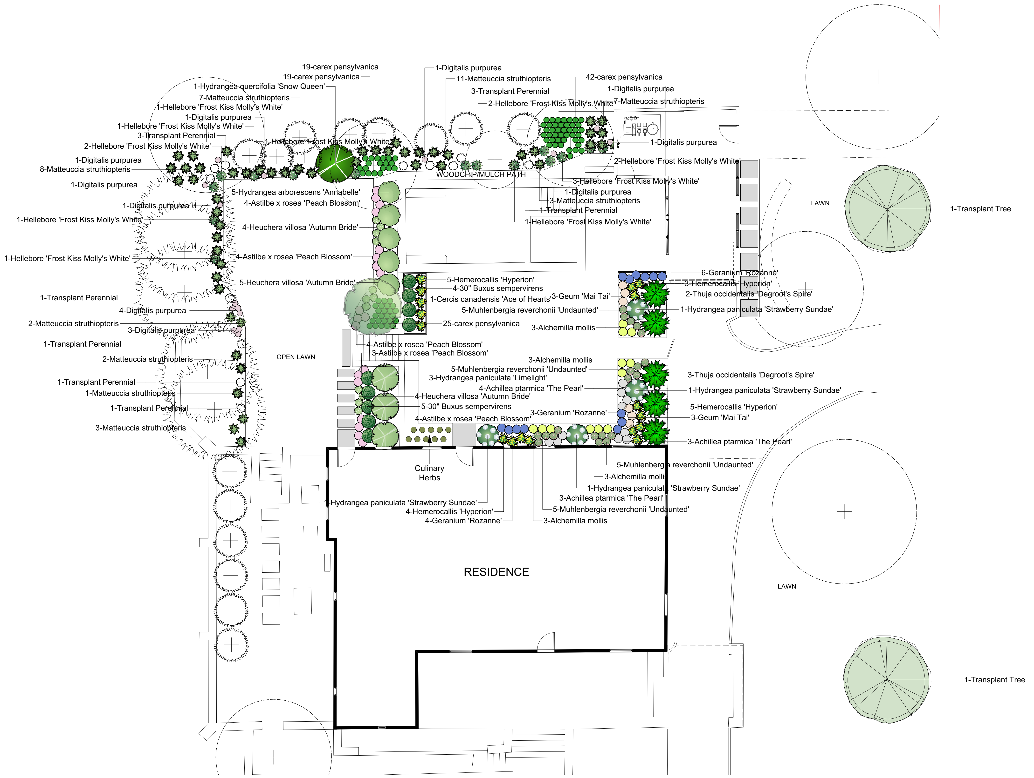
1 PLANTING PLAN Scale: 1/8" = 1'-0"
