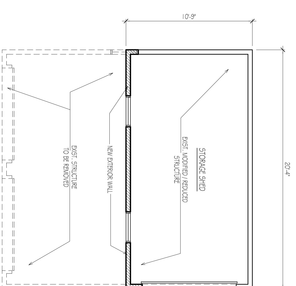
5. SHED PLAN V-4 SCALE: 1/8" = 1'-0"
