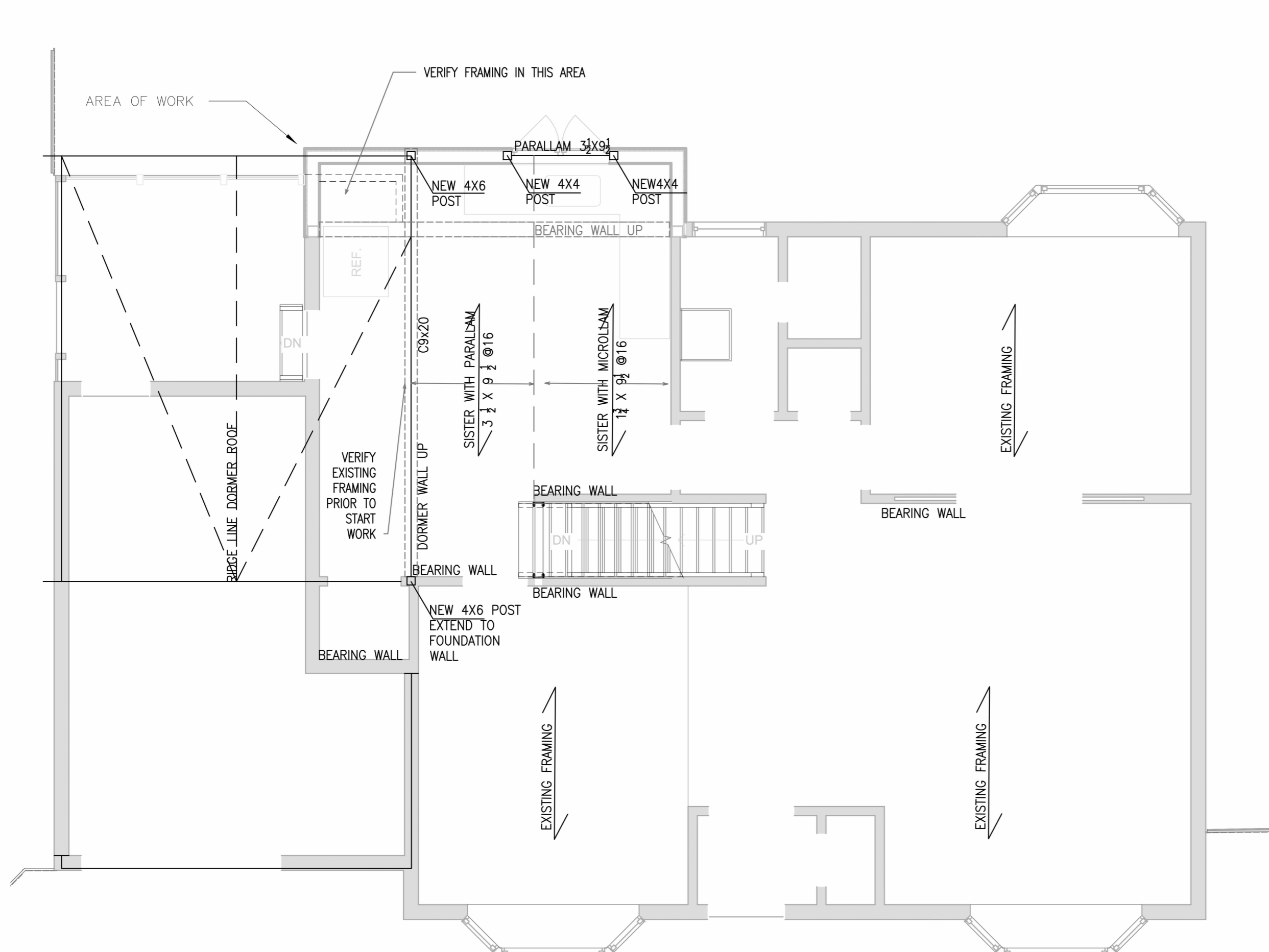
SECOND FLOOR FRAMING PLAN
