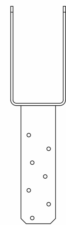
SIMPSON ECCQ44SDS2.5 COLUMN CAP
