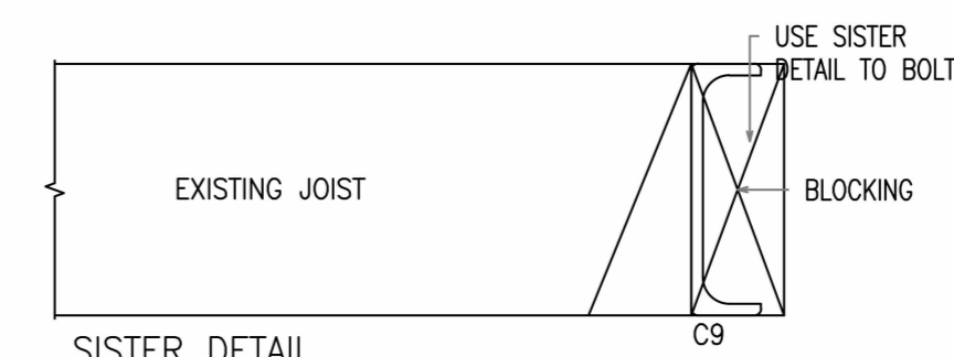
SISTER DETAIL
