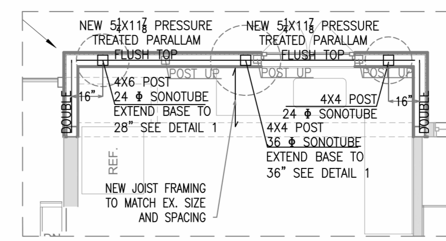
FIRST/FOUNDATION PART PLAN
